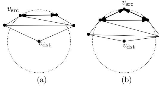
FIG. 2.2. Triangulations that defeat the greedy routing algorithm.
