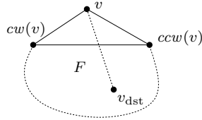
FIG. 2.8. The proof of Theorem 2.6.
