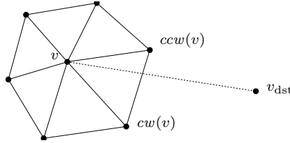
FIG. 2.7. Definition of cw(v) and ccw(v) .
