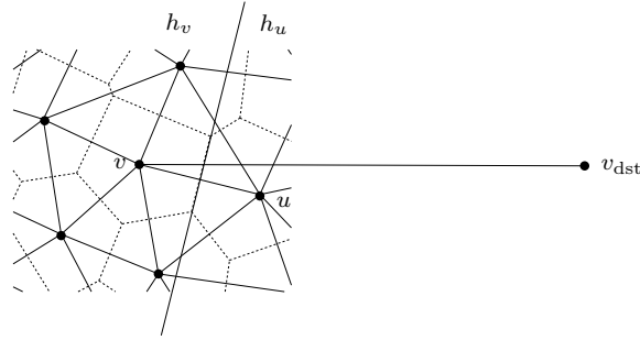
FIG. 2.3. The proof of Theorem 2.2.
